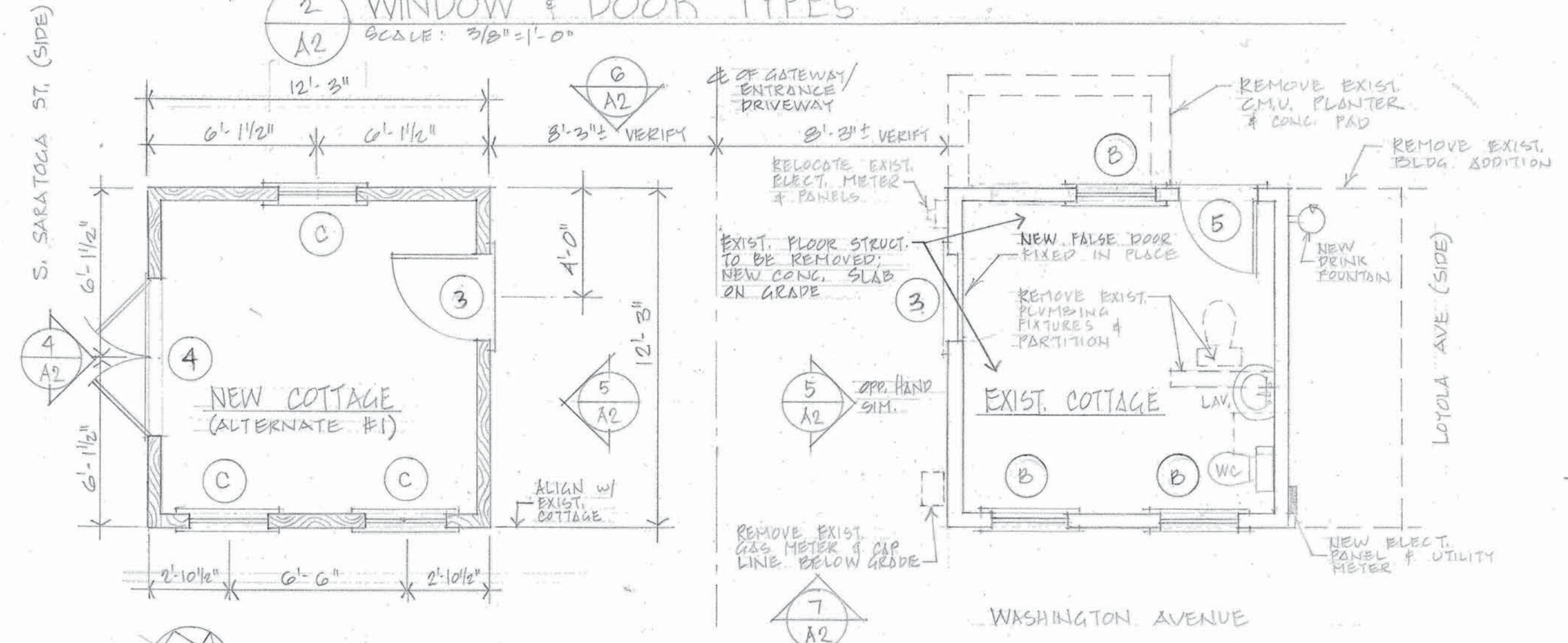
3 FLOOR PLAN SCALE: 1/4" = 1'-0"
