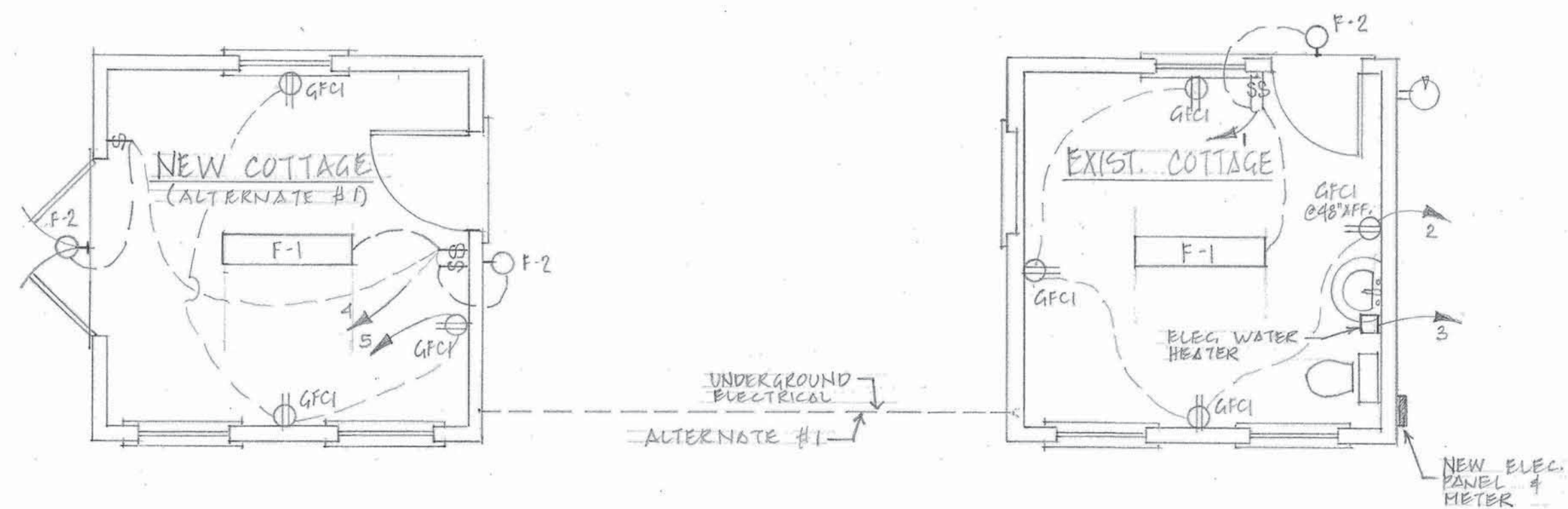
2 ELECTRICAL FLOOR PLAN - LAFAYETTE No. 2 SCALE: 1/4" = 1'-0"
