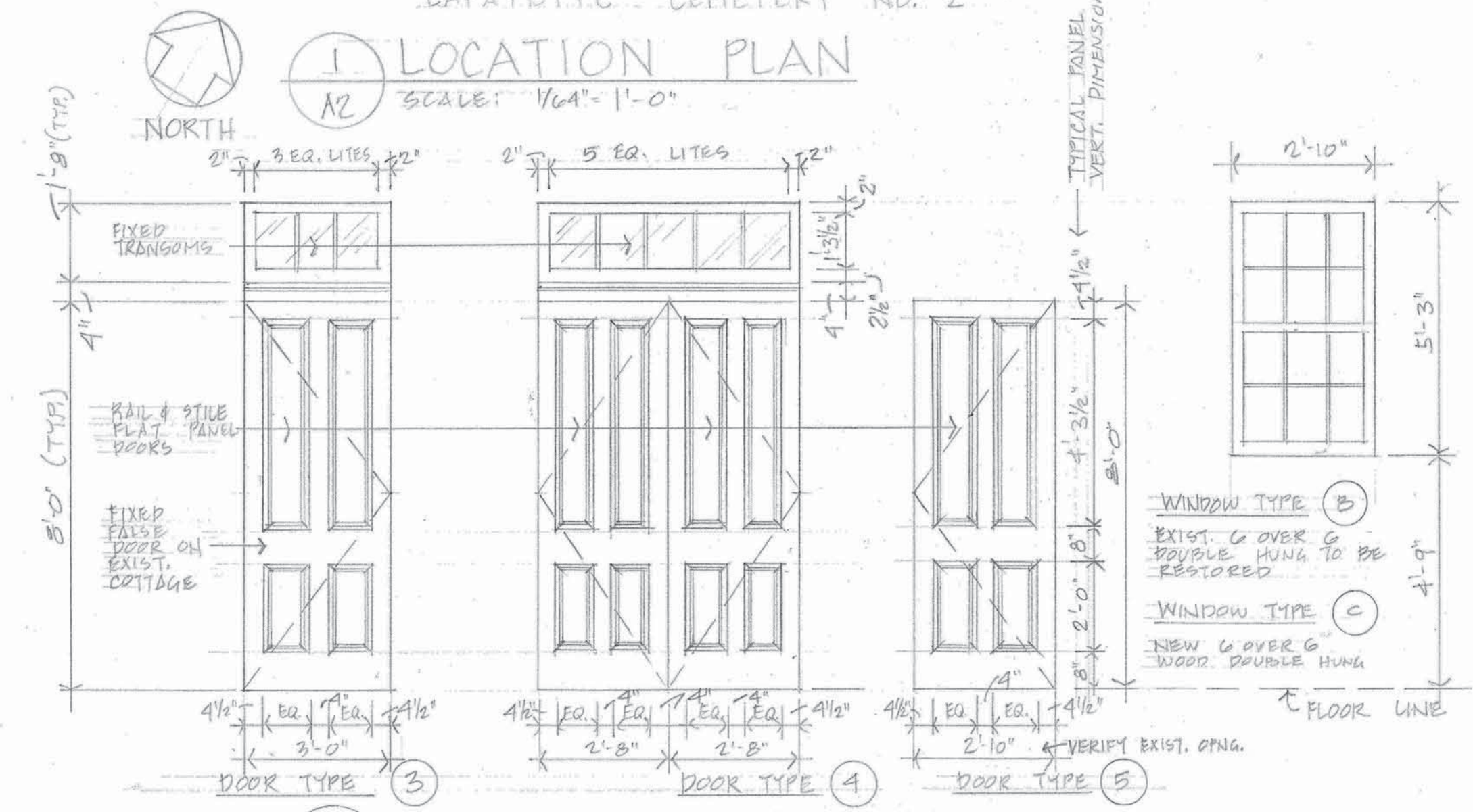
2 WINDOW & DOOR TYPES SCALE: 3/8" = 1'-0"
