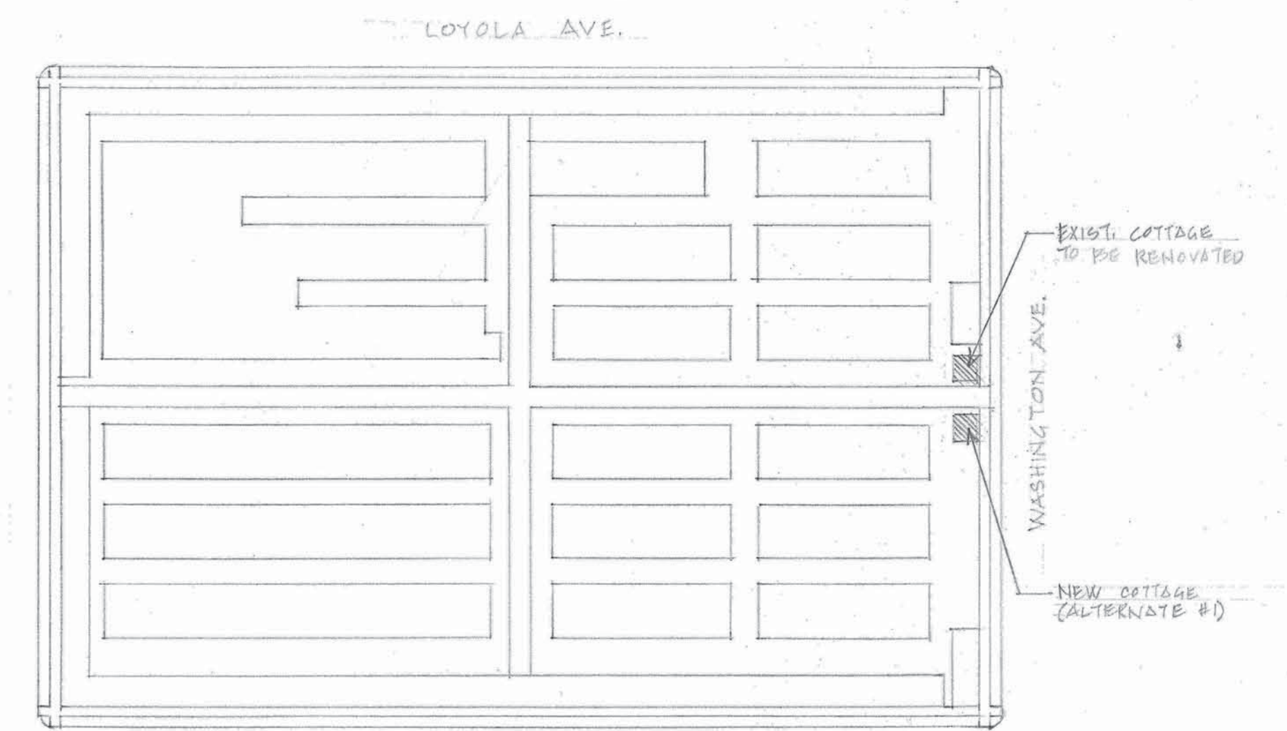
1 LOCATION PLAN SCALE: 1/64" = 1'-0"
