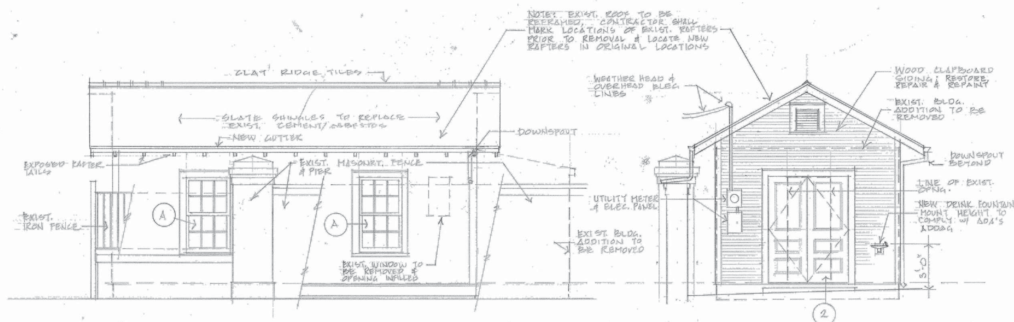
4 SIXTH STREET (SIDE) ELEVATION A1 SCALE: 1/4" = 1'-0"
