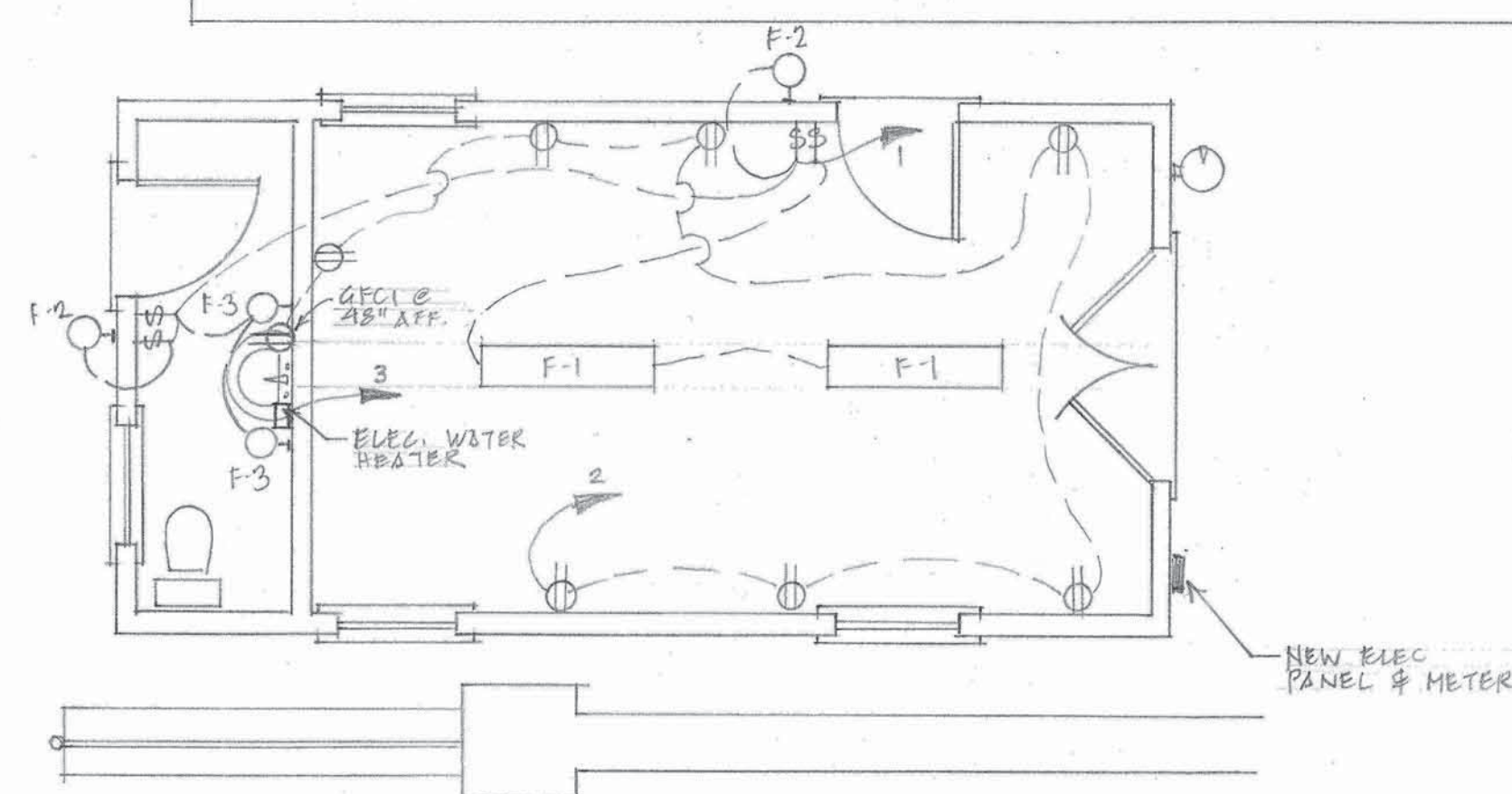
1 ELECTRICAL FLOOR PLAN - LAFAYETTE No. 1 SCALE: 1/4" = 1'-0"
