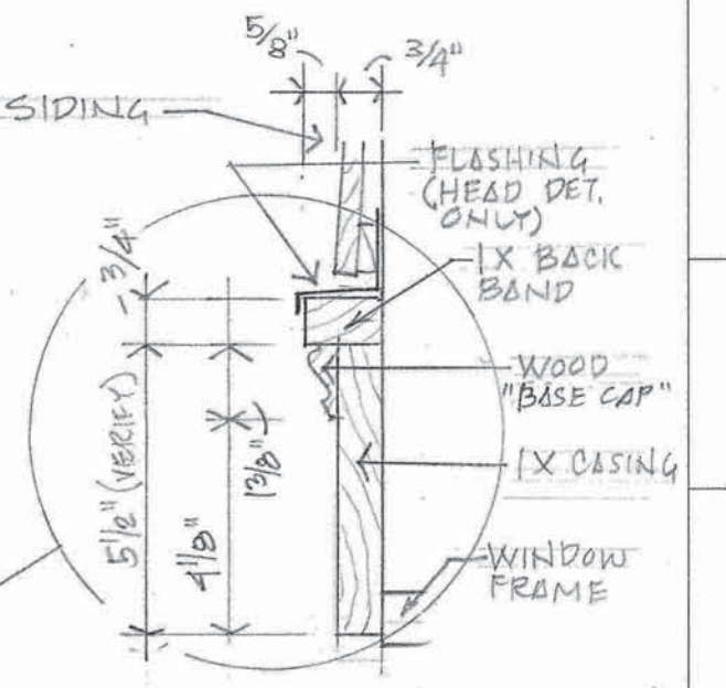
TYP. WOOD TRIM SCALE: 3/8" = 1'-0" (LAFAYETTE #2 ONLY) NOTE: JAMB DET. SIMILAR
